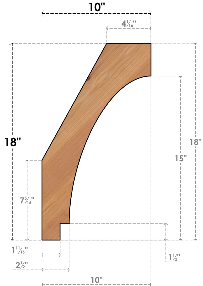
SIDE
